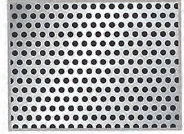
PATTERN No.6 1/4 Diam. 1.4 mm. Pitch 2.28 mm. Open Area 36.75%
