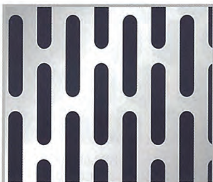
PATTERN No.SL-37520 Diam. 3.75 x 20 mm. Pitch 1 - 7.00 mm. Pitch 2 - 23.50 mm. Open Area 43.75%
