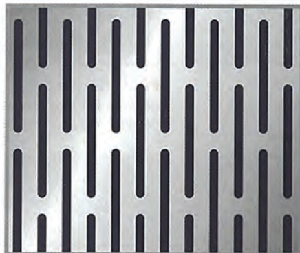
PATTERN No.SL-1520 Diam. 1.5 x 20 mm. Pitch 1 - 4 mm. Pitch 2 - 23.50 mm. Open Area 31.40%
