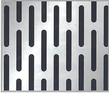
PATTERN No.SL-2520 Diam. 2.5 x 20 mm. Pitch 1 - 6.00 mm. Pitch 2 - 23.50 mm. Open Area 34.51%
