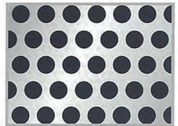
PATTERN No.11 1/4 Diam. 4.5 mm. Pitch 6.4 mm. Open Area 45%
