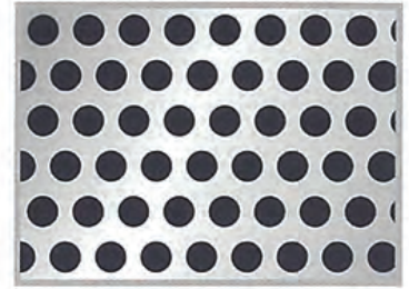
PATTERN No.10 1/4 Diam. 3.4 mm. Pitch 5.00 mm. Open Area 42%
