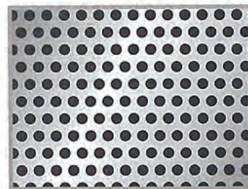
PATTERN No.7 1/2 Diam. 1.9 mm. Pitch 3.00 mm. Open Area 38%
