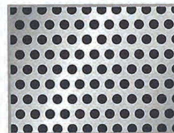
PATTERN No.8 3/4 Diam. 2.4 mm. Pitch 3.60 mm. Open Area 40.31%
