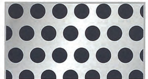
PATTERN No.12 3/4 Diam. 6.25 mm. Pitch 9.0 mm. Open Area 44%
