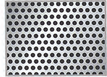
PATTERN No.7 1/4 Diam. 1.8 mm. Pitch 2.72 mm. Open Area 40%
