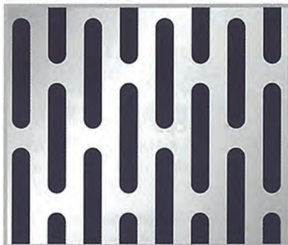
PATTERN No.SL-32520 Diam. 3.25 x 20 mm. Pitch 1 - 6.50 mm. Pitch 2 - 23.50 mm. Open Area 41%
