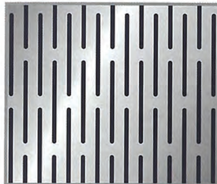
PATTERN No.SL-1020 Diam. 1 x 20 mm. Pitch 1 - 3 mm. Pitch 2 - 23.50 mm. Open Area 28%
