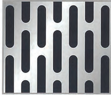
PATTERN No.SL-4020 Diam. 4 x 20 mm. Pitch 1 - 7.50 mm. Pitch 2 - 23.50 mm. Open Area 44%
