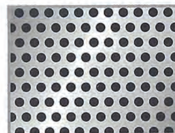
PATTERN No.8 1/2 Diam. 2.3 mm. Pitch 3.67 mm. Open Area 36%
