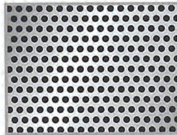
PATTERN No.6 3/4 Diam. 1.6 mm. Pitch 2.46 mm. Open Area 38%
