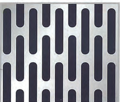
PATTERN No.SL-3520 Diam. 3.5 x 20 mm. Pitch 1 - 6.85 mm. Pitch 2 - 23.50 mm. Open Area 42%
