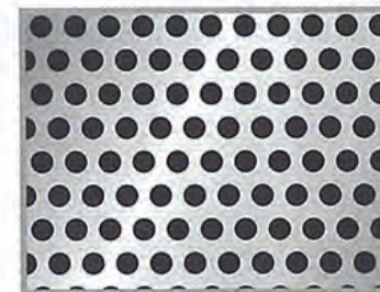
PATTERN No.9 Diam. 2.5 mm. Pitch 3.80 mm. Open Area 39%
