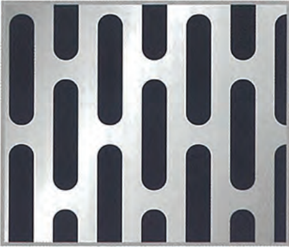
PATTERN No.SL-4520 Diam. 4.5 x 20 mm. Pitch 1 - 8.00 mm. Pitch 2 - 23.50 mm. Open Area 45.55%
