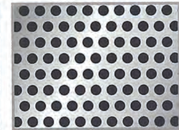
PATTERN No.9 1/4 Diam. 2.65 mm. Pitch 4.0 mm. Open Area 40%
