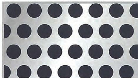
PATTERN No.12 1/2 Diam. 6.0 mm. Pitch 8.5 mm. Open Area 45%
