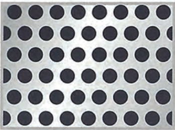
PATTERN No.10 1/2 Diam. 3.6 mm. Pitch 5.2 mm. Open Area 44%
