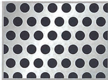
PATTERN No.10 3/4 Diam. 3.8 mm. Pitch 5.5 mm. Open Area 43%
