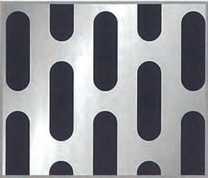
PATTERN No.SL-6020 Diam. 6 x 20 mm. Pitch 1 - 11.00 mm. Pitch 2 - 25.00 mm. Open Area 40.82%
