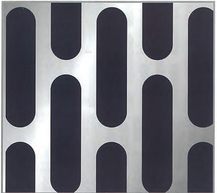
PATTERN No.SL-12750 Diam. 12.7 x 50 mm. Pitch 1 - 19.00 mm. Pitch 2 - 56.00 mm. Open Area 56.42%
