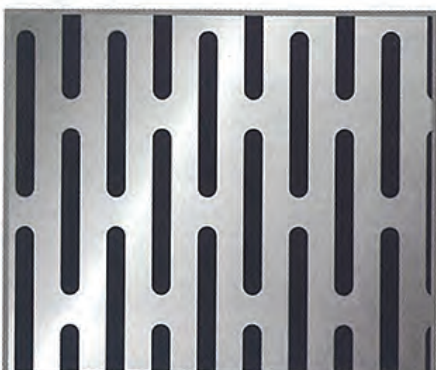
PATTERN No.SL-22520 Diam. 2.25 x 20 mm. Pitch 1 - 5.50 mm. Pitch 2 - 23.50 mm. Open Area 34%
