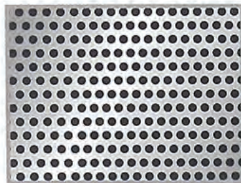
PATTERN No.6 1/2 Diam. 1.5 mm. Pitch 2.46 mm. Open Area 34%
