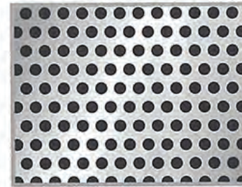
PATTERN No.8 Diam. 2.1 mm. Pitch 3.30 mm. Open Area 37%
