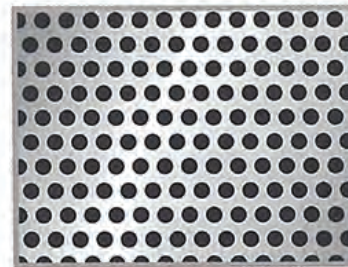
PATTERN No.7 3/4 Diam. 2.00 mm. Pitch 3.00 mm. Open Area 40%
