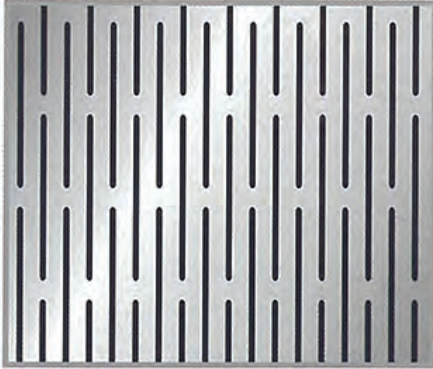
PATTERN No.SL-0720 Diam. 0.7 x 20 mm. Pitch 1 - 2.80 mm. Pitch 2 - 22.30 mm. Open Area 21.57%
