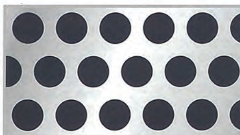
PATTERN No.13 1/2 Diam. 7.5 mm. Pitch 10.4 mm. Open Area 47%
