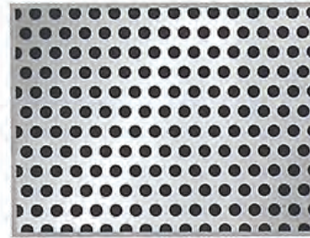
PATTERN No.7 Diam. 1.7 mm. Pitch 2.72 mm. Open Area 36%
