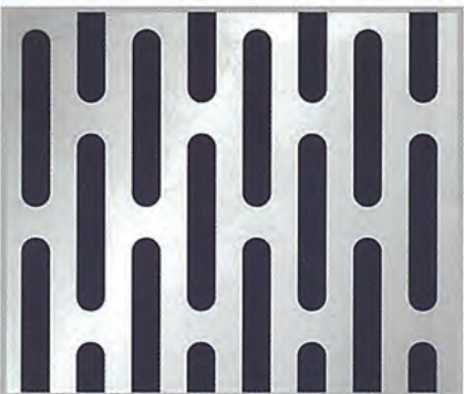
PATTERN No.SL-3220 Diam. 3.2 x 20 mm. Pitch 1 - 6.25 mm. Pitch 2 - 23.50 mm. Open Area 42%
