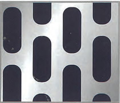
PATTERN No.SL-8020 Diam. 8 x 20 mm. Pitch 1 - 13.00 mm. Pitch 2 - 25.00 mm. Open Area 45%
