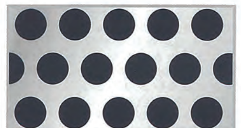
PATTERN No.14 Diam. 8.0 mm. Pitch 11.1 mm. Open Area 47%
