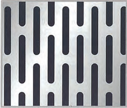
PATTERN No.SL-27520 Diam. 2.75 x 20 mm. Pitch 1 - 6.00 mm. Pitch 2 - 23.50 mm. Open Area 37.85%
