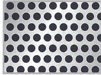
PATTERN No.10 Diam. 3.2 mm. Pitch 4.52 mm. Open Area 45%
