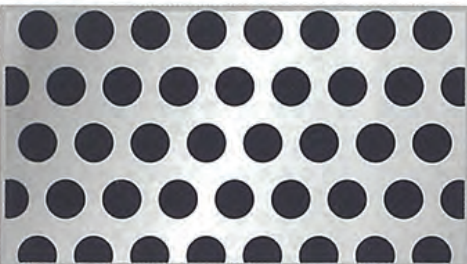
PATTERN No.11 1/2 Diam. 4.8 mm. Pitch 6.9 mm. Open Area 44%
