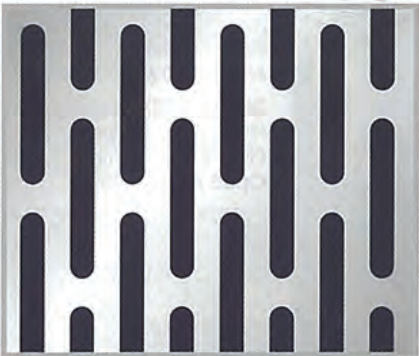
PATTERN No.SL-3020 Diam. 3 x 20 mm. Pitch 1 - 6.25 mm. Pitch 2 - 23.50 mm. Open Area 40%
