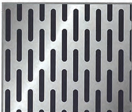
PATTERN No.SL-2013 Diam. 2 x 13 mm. Pitch 1 - 4.50 mm. Pitch 2 - 16.00 mm. Open Area 35%
