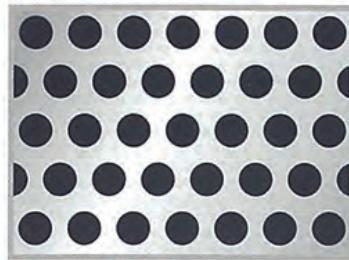
PATTERN No.11 Diam. 4.1 mm. Pitch 6.0 mm. Open Area 42%
