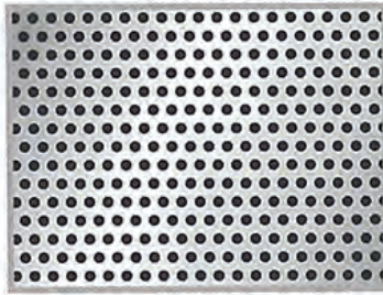
PATTERN No.5 1/2 Diam. 1.2 mm. Pitch 2.06 mm. Open Area 31%
