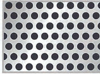
PATTERN No.9 3/4 Diam. 3.00 mm. Pitch 4.4 mm. Open Area 42%
