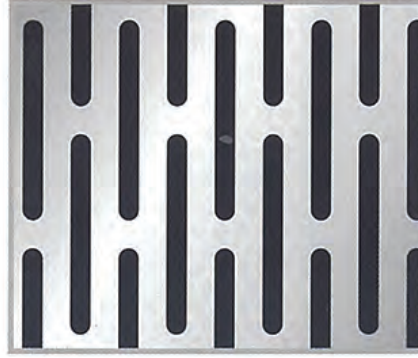
PATTERN No.SL-2525 Diam. 2.5 x 25 mm. Pitch 1 - 6.00 mm. Pitch 2 - 28.50 mm. Open Area 35%
