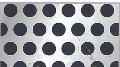
PATTERN No.13 Diam. 6.5 mm. Pitch 9.2 mm. Open Area 45%
