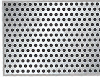
PATTERN No.6 Diam. 1.3 mm. Pitch 2.20 mm. Open Area 32%
