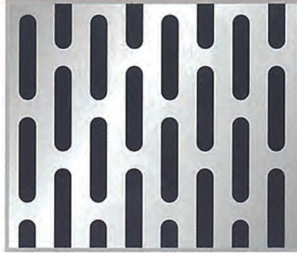
PATTERN No.SL-3015 Diam. 3 x 15 mm. Pitch 1 - 6.25 mm. Pitch 2 - 18 mm. Open Area 32.28%
