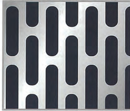
PATTERN No.SL-5020 Diam. 5 x 20 mm. Pitch 1 - 8.35 mm. Pitch 2 - 23.50 mm. Open Area 48%
