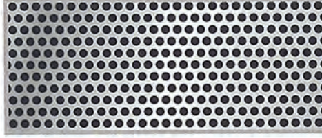
PATTERN No.SKR-15 Diam. 1.5 mm. Pitch 2.1 mm. Open Area 46.28% Size 300 mm x100 m (Coil) 205 mm x100 m (Coil) 180 mm x100 m (Coil)
