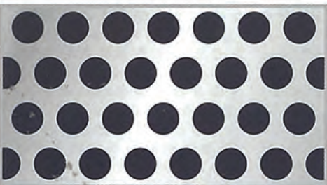
PATTERN No.12 1/4 Diam. 5.6 mm. Pitch 7.92 mm. Open Area 45%
